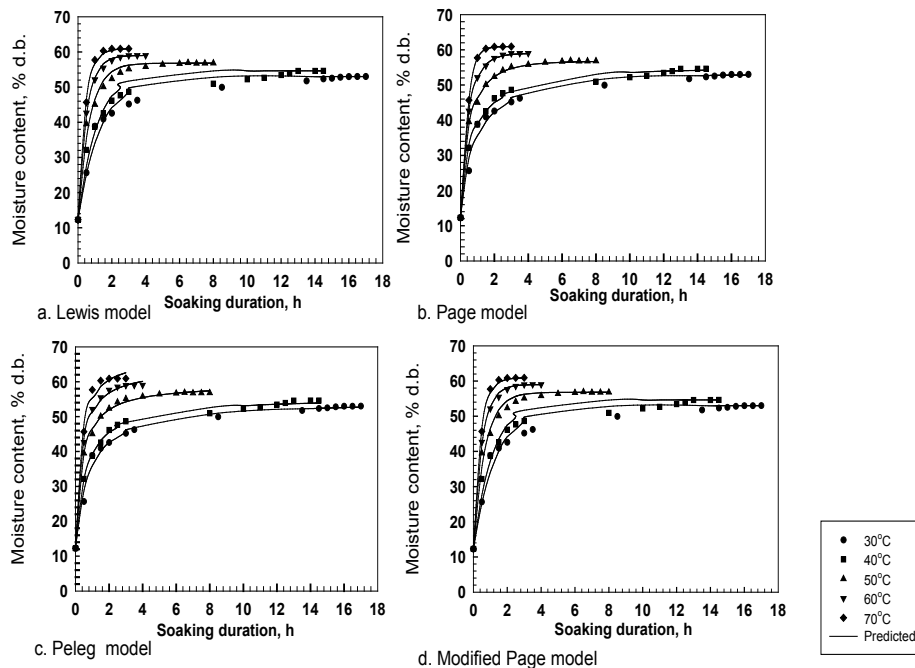
Fig. 1. Hydration characteristics of finger millet grains
