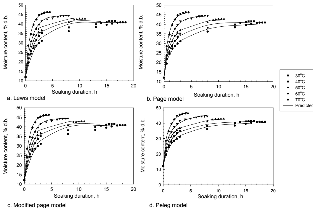
Fig. 2. Hydration characteristics of foxtail millet grains
